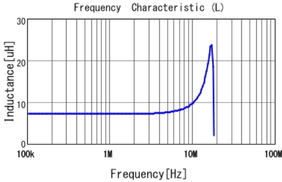
DFE322512F-6R8M L
