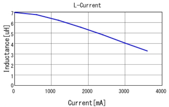
DFE322512F-6R8M L-Current 20degC
