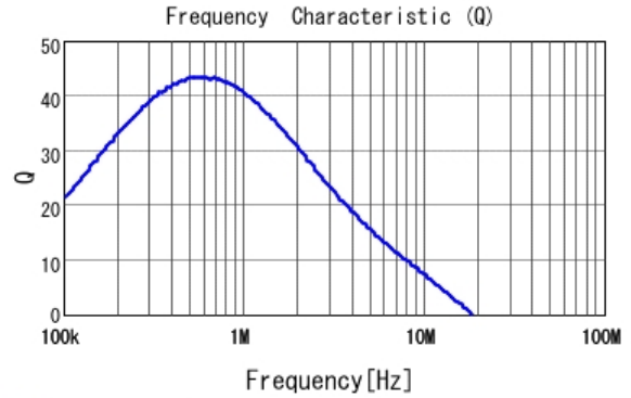
DFE322512F-6R8M Q
