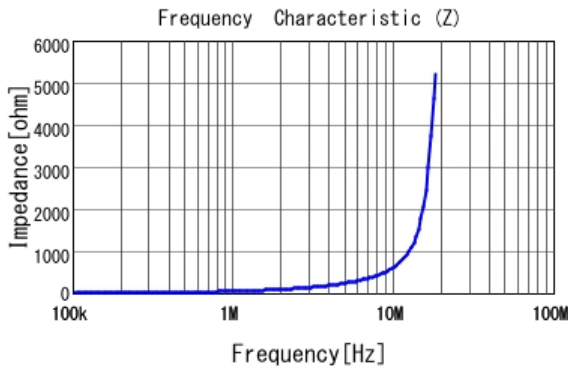
DFE322512F-6R8M |Z|
